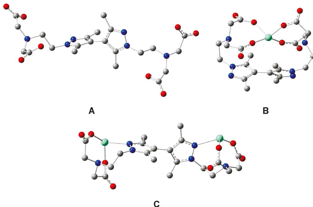
Figure 4. Optimized structures of biazolic complexone 5b calculated in the absence (A) and presence of one (B) or two (C) Gd(III) atoms. Calculations were performed using the HF/3-21G basis set for the ligand, and the 46 + 4f 7 ECP with the [5s4p3d]-GTO valence basis set for the metal, as indicated in the Experimental. The Gd(III) atoms are shown in green.
