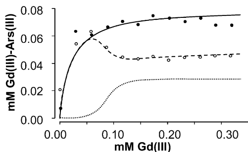
Figure 3. Binding of Gd(III) to ArsIII in the absence (solid lines) or presence (dashed line) of 5a . Sigmoidal Gd(III) binding to 5a (dotted line) is calculated as the difference between the solid and dashed lines. Binding parameters S_{0.5} and n reflecting the half maximal saturation of the complexone and the degree of cooperativity can be estimated as indicated in the Experimental (c.f. Table 1).
