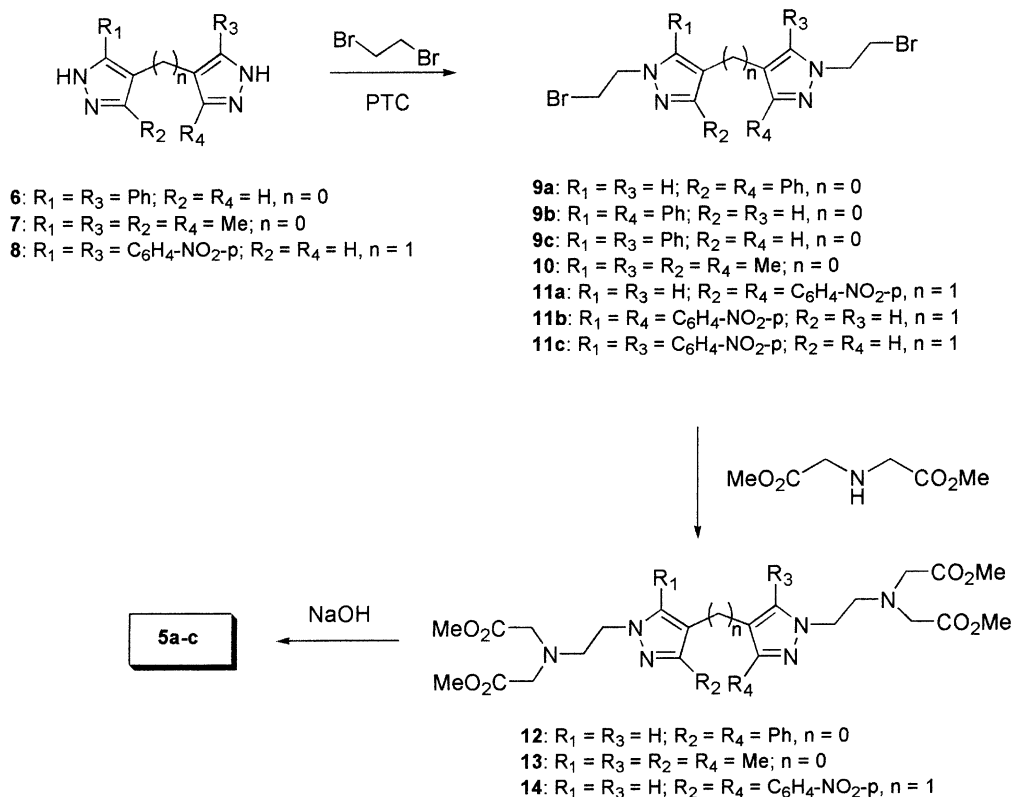
Scheme 1. Syntheses of complexones 5a–c .
