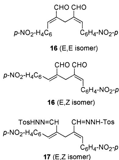
Figure 2. Structures of the isomers of 16 and 17 .
