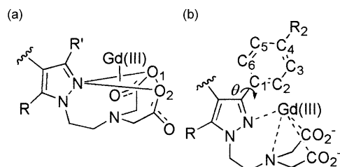
Figure 5. Coordination geometry around the metal in 5a–d complexes: (a) distance from the metal to the N–O1–O2 plane of the ligand; (b) effect of the phenyl ring.
