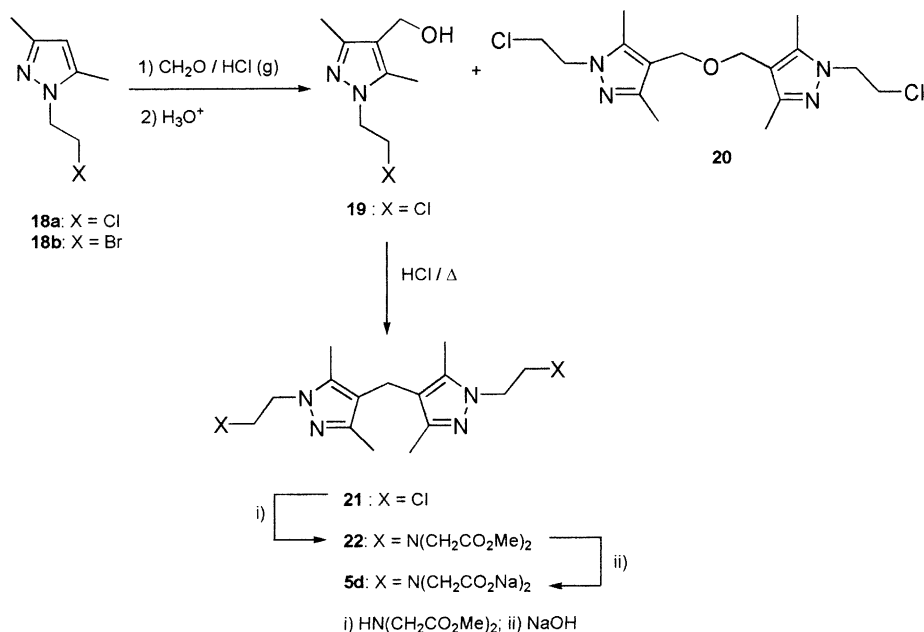
Scheme 2. Synthesis of complexone 5d .
