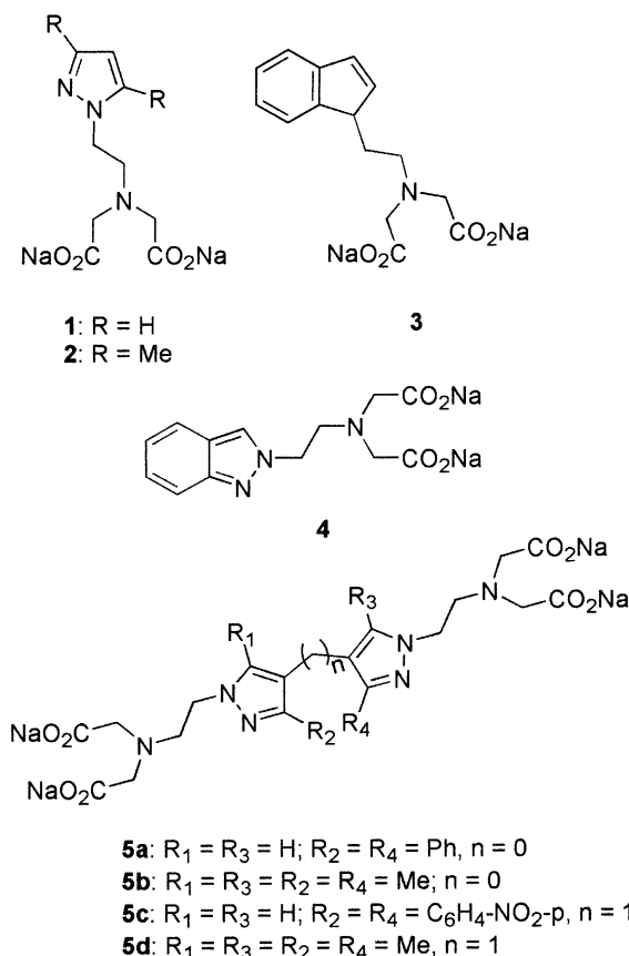
Figure 1. Structures of monoazolic complexones 1–4 12 and bis- or biazolic complexones 5a–d .
