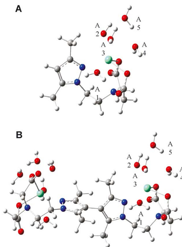
Figure 6. Calculated structures of 2 (A) and 5b (B) in the presence of five water molecules (A1–A5) in the inner coordination sphere of Gd(III). Note that A5 is excluded from the coordination center. Calculations were performed as in Figure 4.
